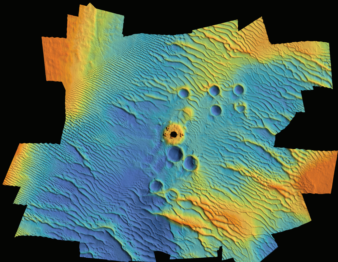
Title: Offshore wind turbine with adjacent spudcan footprints Submitted by: Njord Survey Product: EM2040-04 Dual RX
